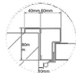
Frame dimensions
